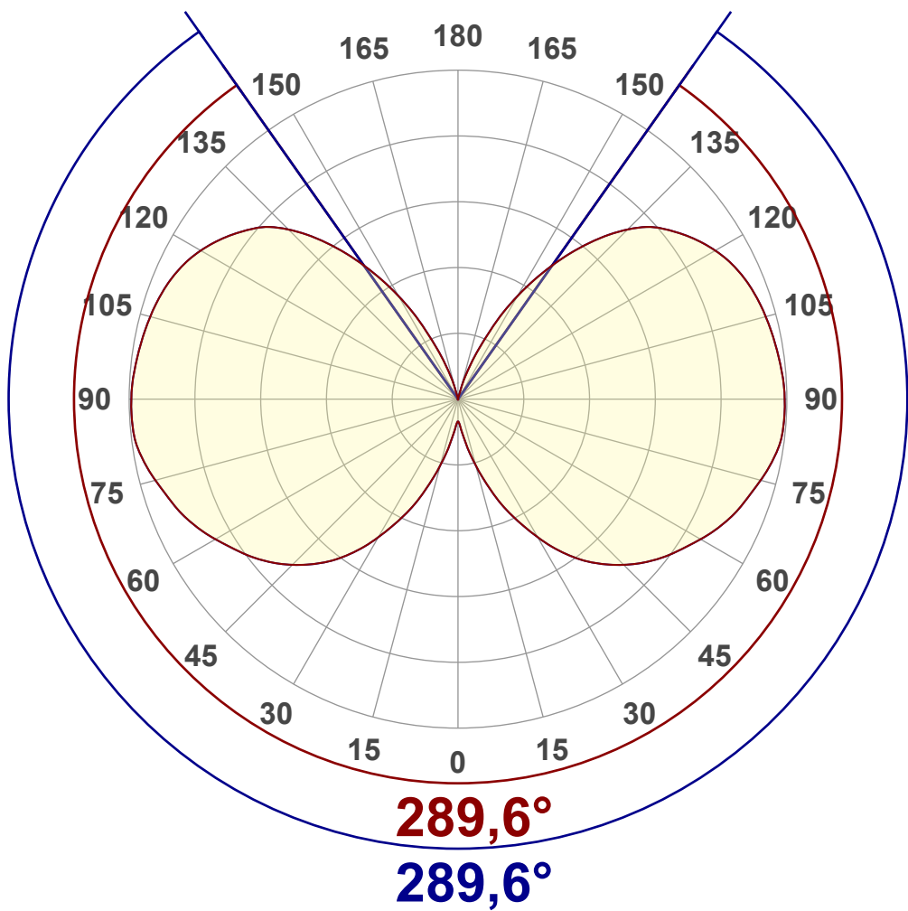
Linear distribution diagram - Intensity (candela) vs γ-angle
